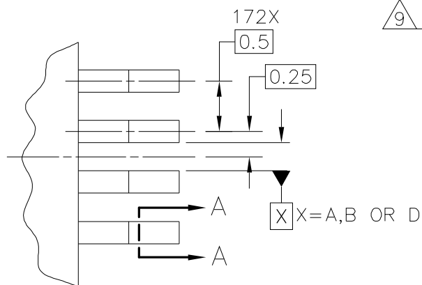
DETAIL K
