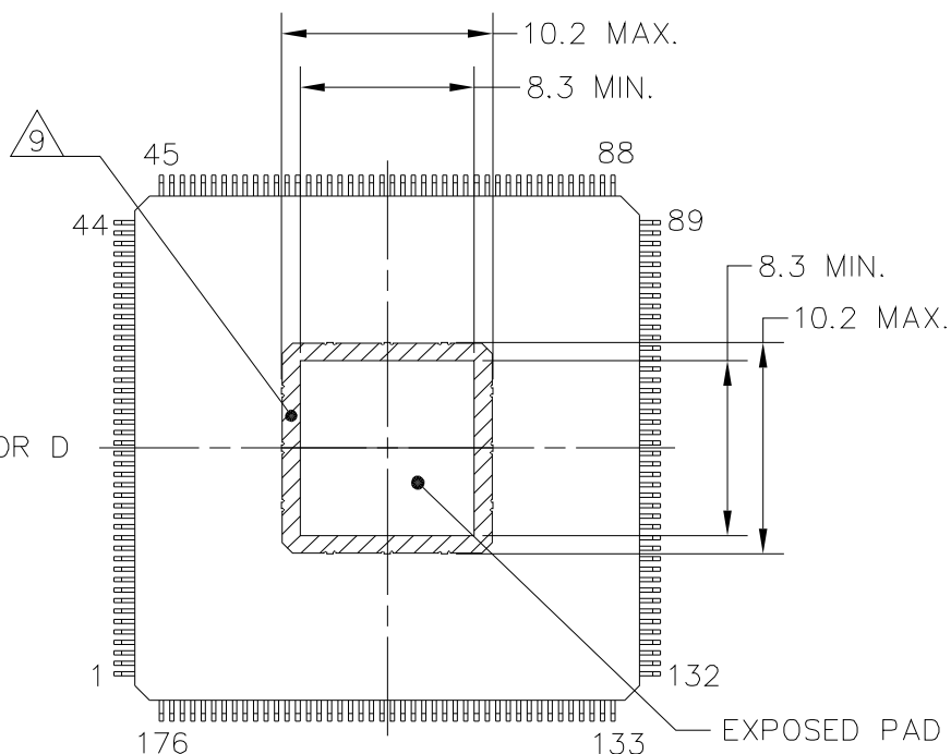
VIEW J-J
