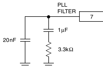
MCVVQ111 loop filter components.
