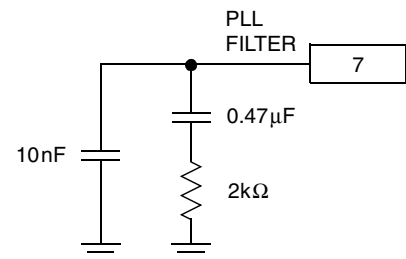
MCVVQ111A loop filter components.
