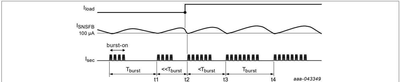
Figure 15. Burst mode: Regulating the number of low-power cycles
