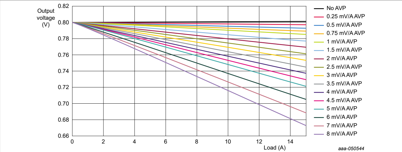
Figure 32. SW1 load regulation at different AVP settings
