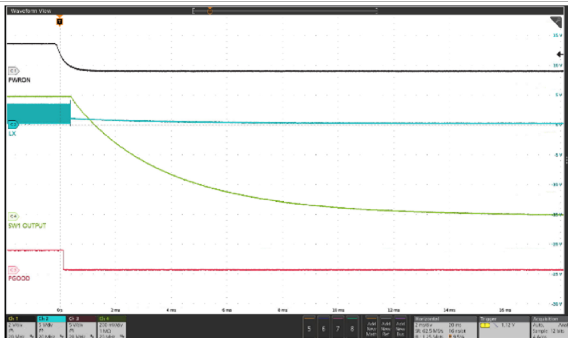
Figure 34. SW1 turn-off with OTP_SW1_RDIS = 1 and OTP_SW1_HIZOFF = 1
