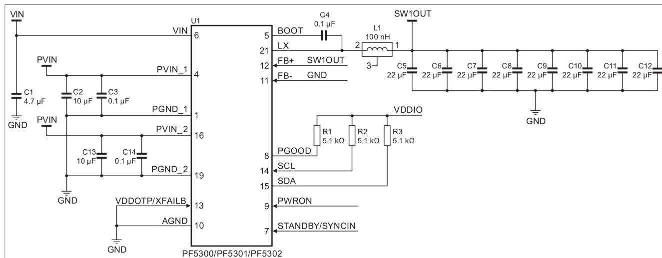
Figure 35. Typical application schematic
