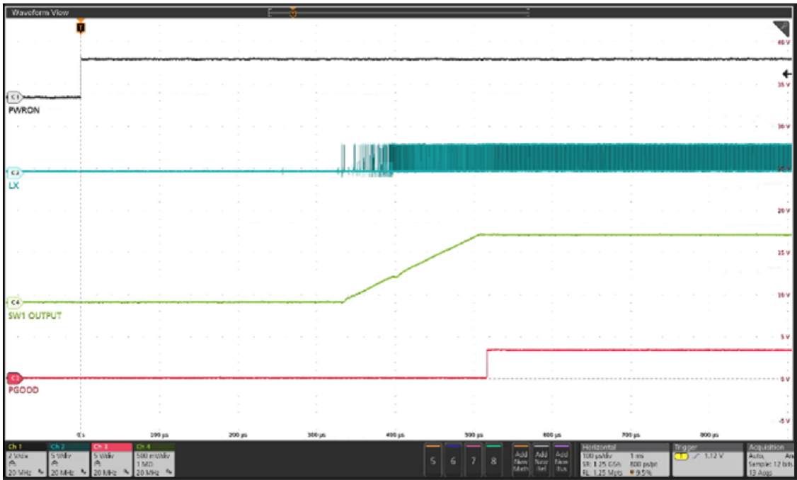
Figure 24. SW1 soft-start (MPF53BDAMMA1ES); 100 \mu s/DIV
