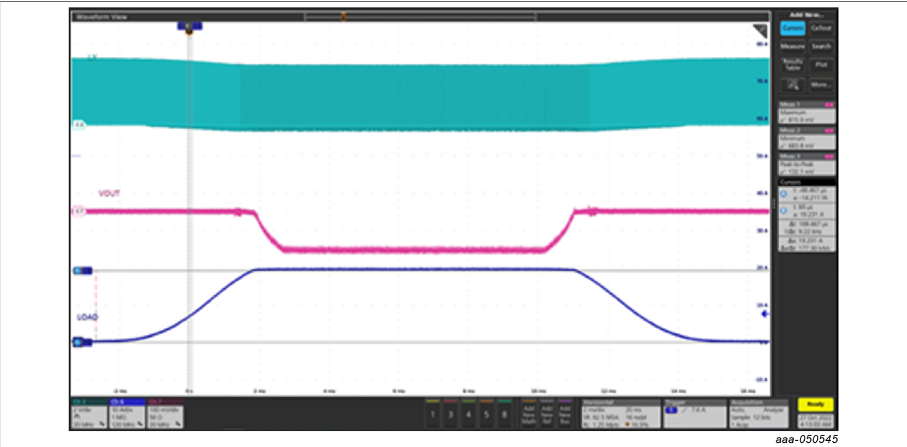
Figure 33. SW1 current limit entry and exit: V out drops and recovers smoothly
