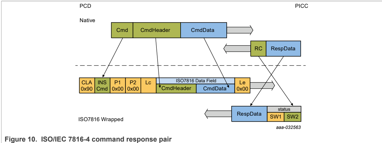
Figure 10. ISO/IEC 7816-4 command response pair
