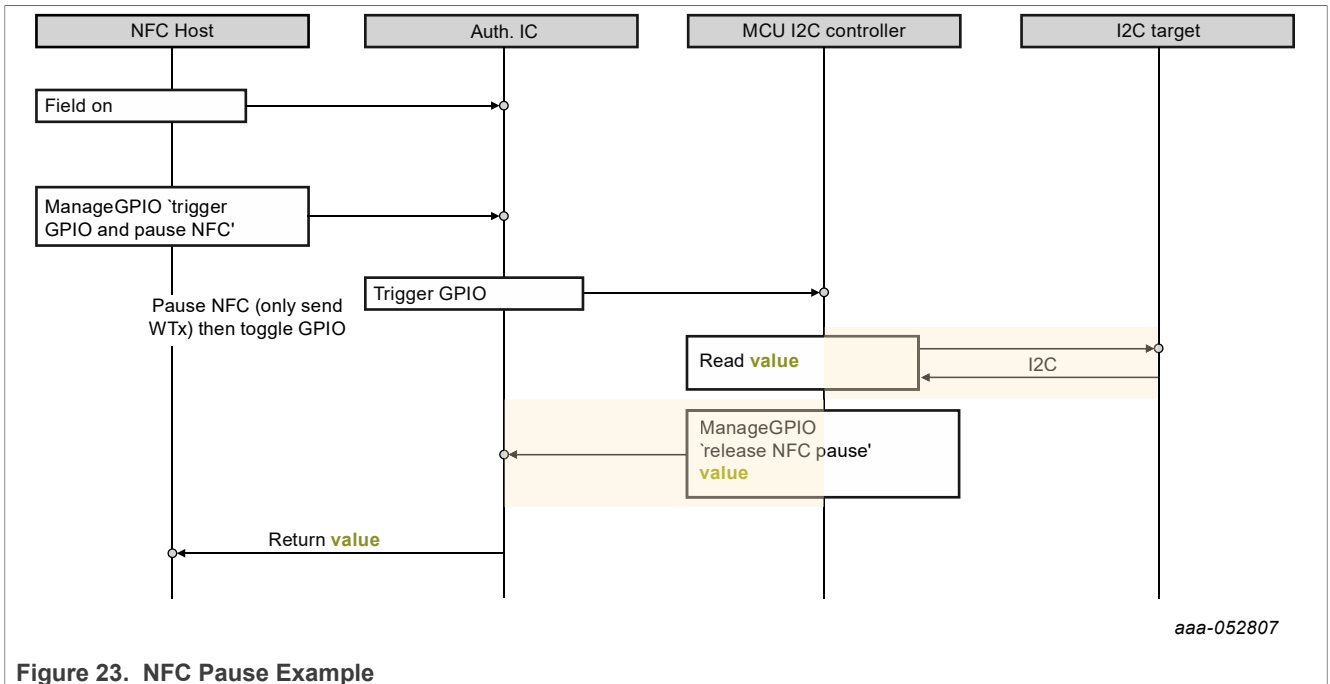
Figure 23. NFC Pause Example
