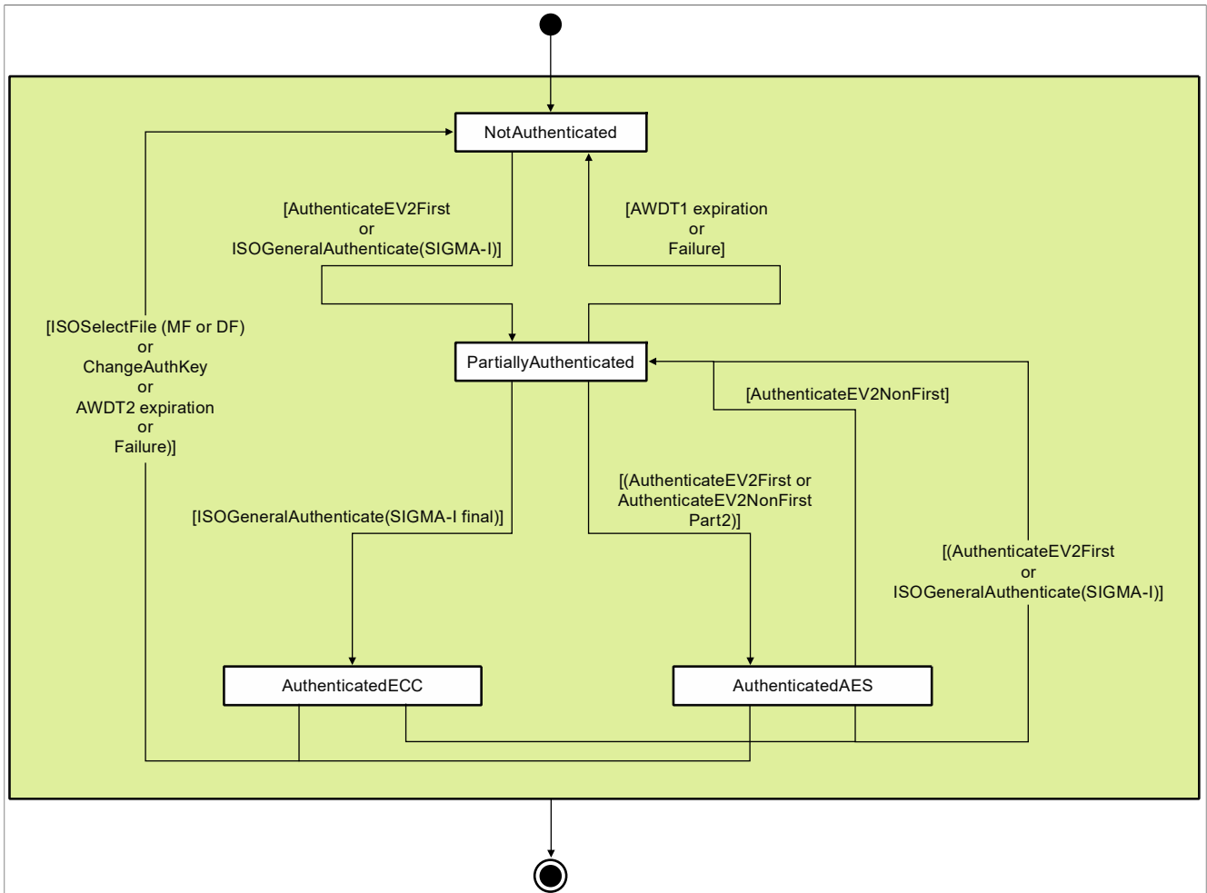
Figure 11. Authentication State Diagram
