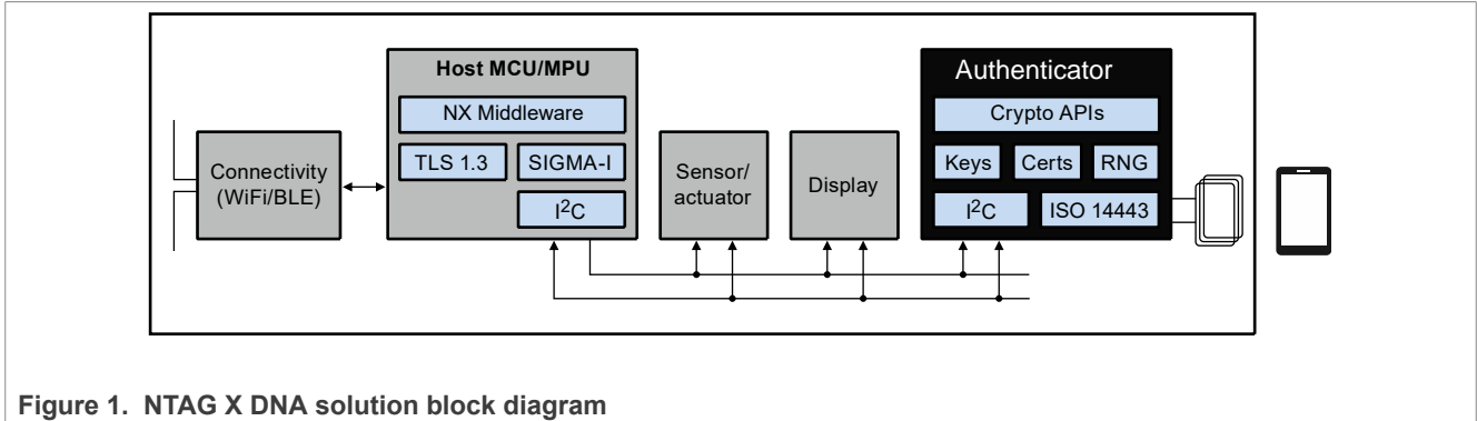
Figure 1. NTAG X DNA solution block diagram
