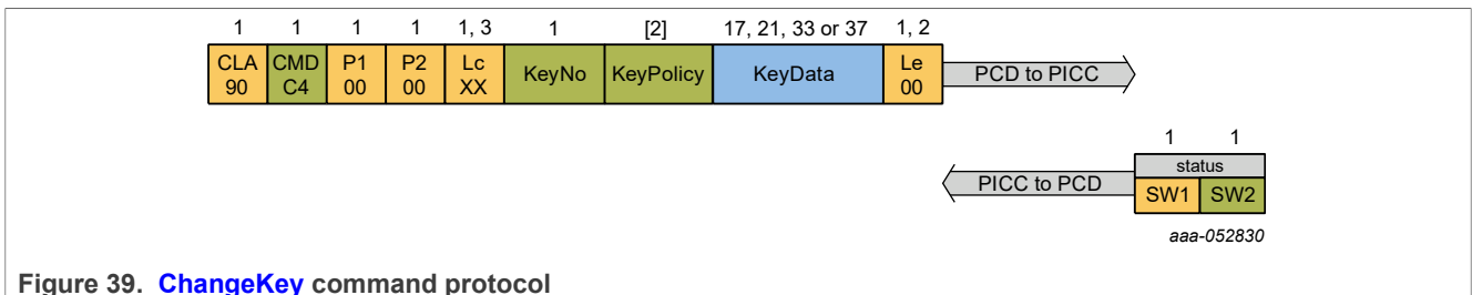
Figure 39. ChangeKey command protocol
