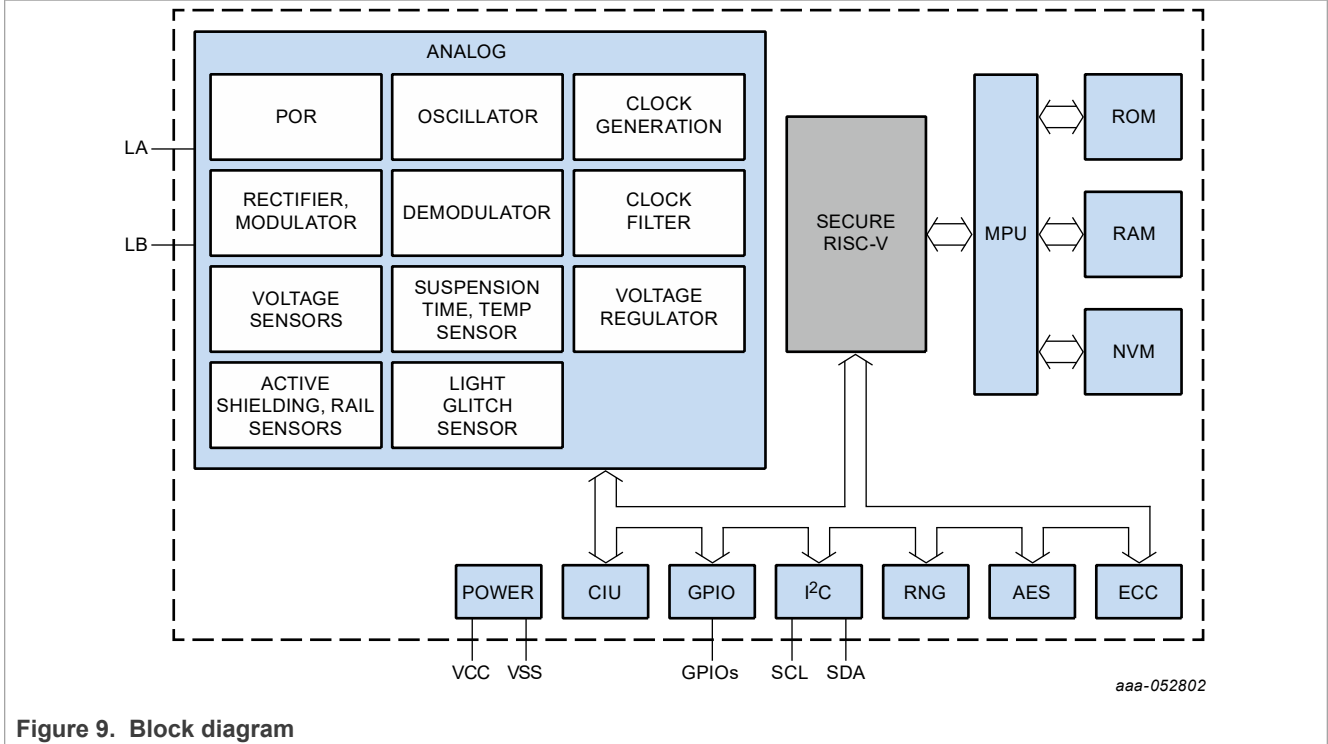
Figure 9. Block diagram
