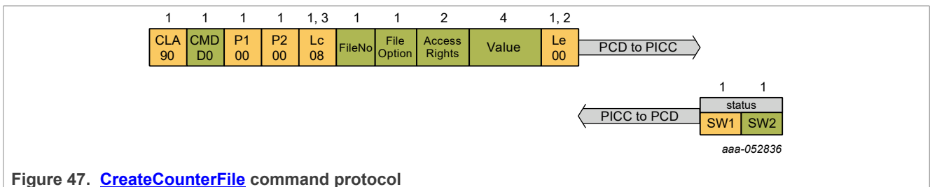
Figure 47. CreateCounterFile command protocol
