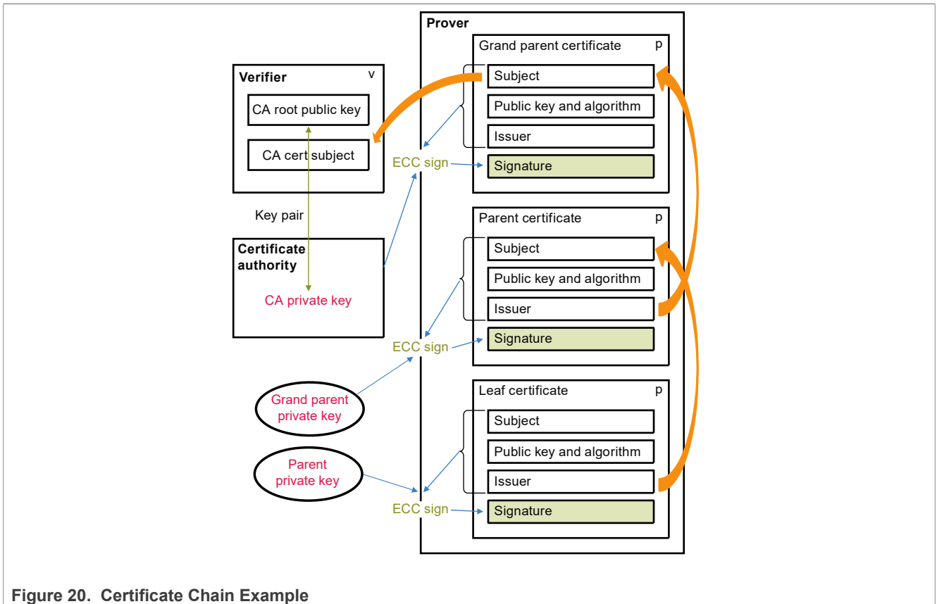
Figure 20. Certificate Chain Example
