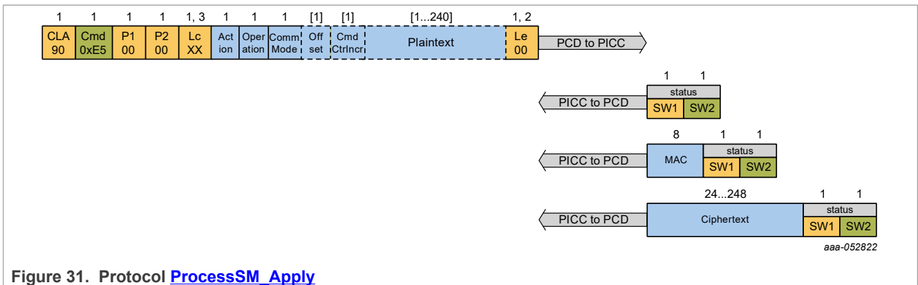
Figure 31. Protocol ProcessSM_Apply
