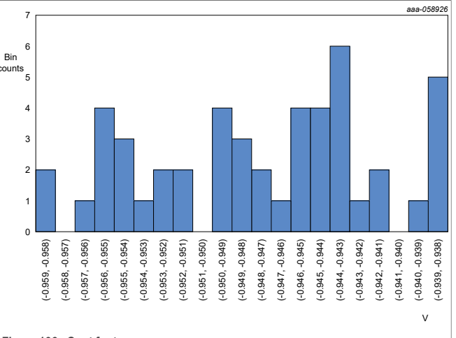
Figure 106. Cout footroom
