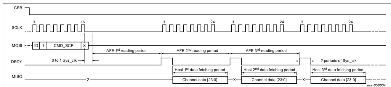
Figure 27. Data capture with CMD_SC method 1
