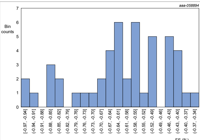
Figure 85. Isense uncalibrated gain error
