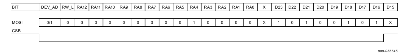
Figure 39. SPI register byte-wise write timing diagram
