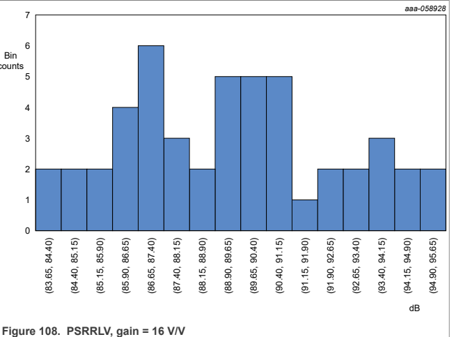
Figure 108. PSRRRLV, gain = 16 V/V
