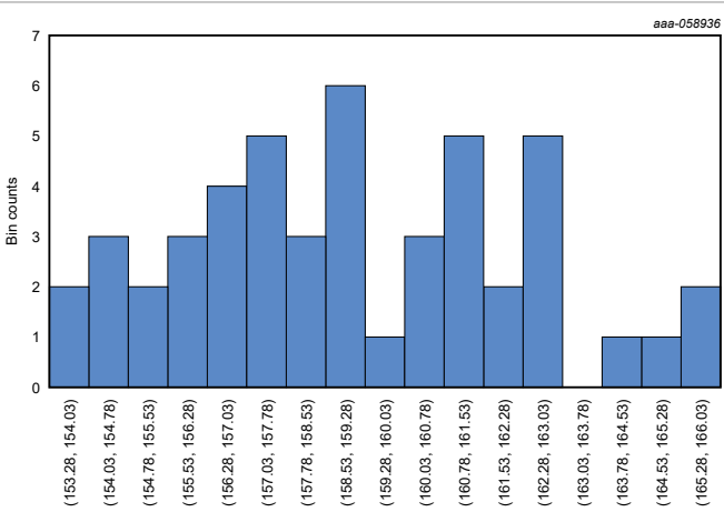
Figure 114. IHVSS at HVSS = -15 V
