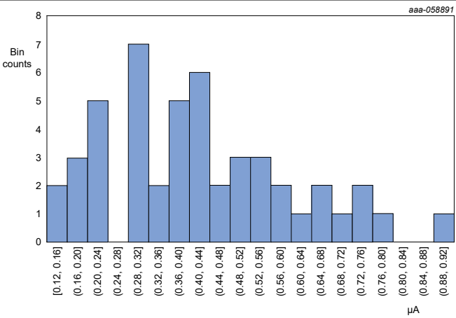
Figure 82. Isense INL
