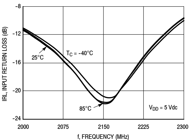
Figure 7. Input Return Loss (S11) versus Frequency
