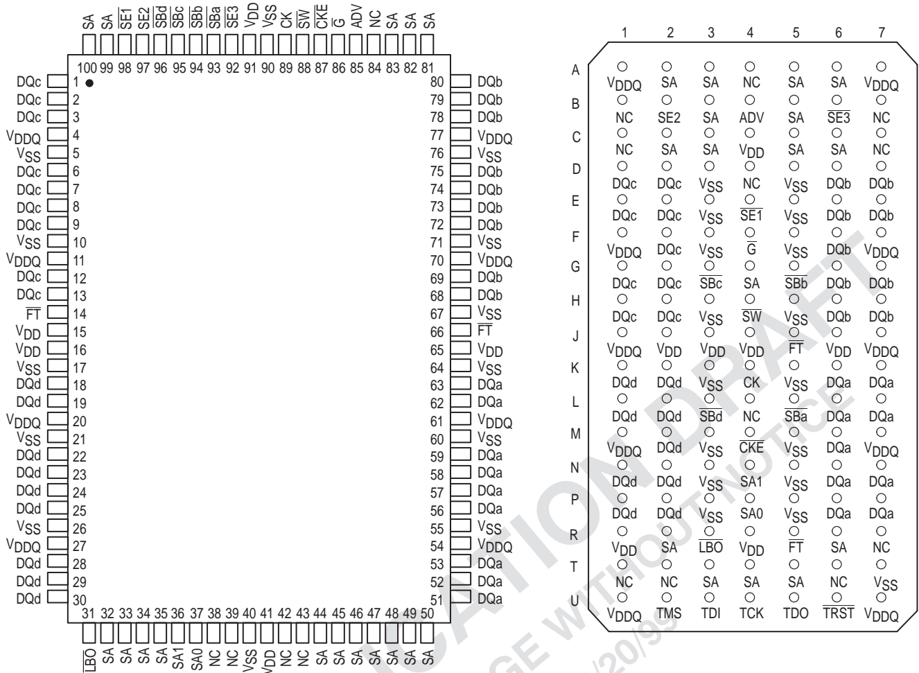
100-PIN TQFP TOP VIEW
