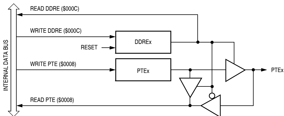
Figure 21-15. Port E I/O Circuit
