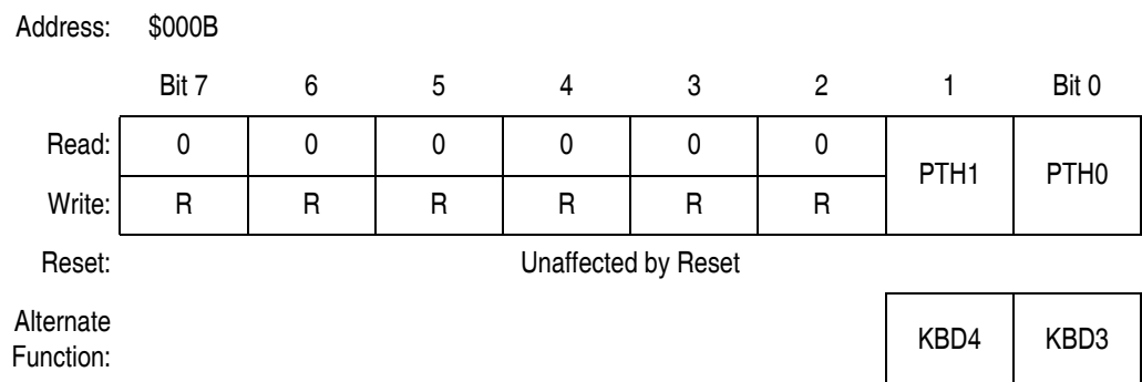
Figure 21-22. Port H Data Register (PTH)
