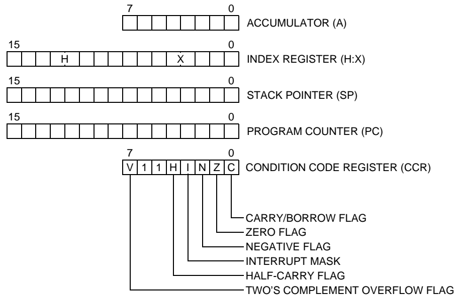
Figure 8-1. CPU registers
