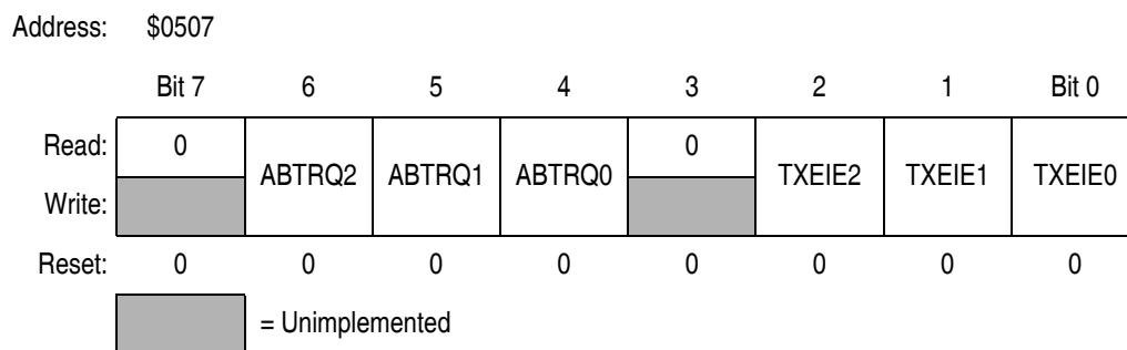
Figure 22-22. Transmitter Control Register (CTCR)
