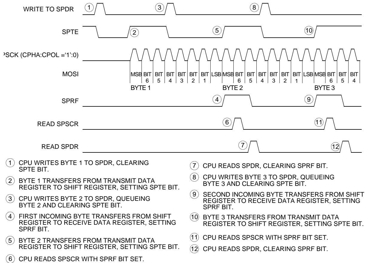
Figure 18-10. SPRF/SPTE CPU Interrupt Timing
