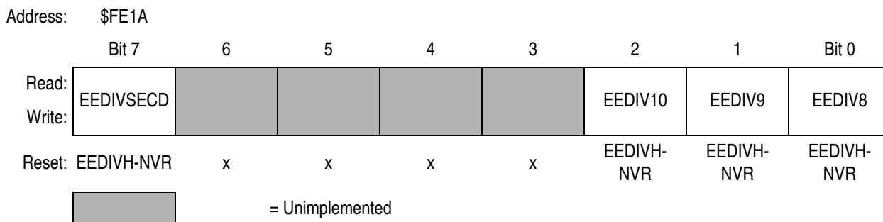
Figure 27-1. EEPROM-2 Divider High Register (EEDIVH)
