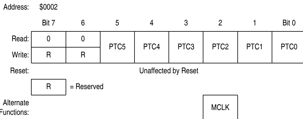
Figure 21-7. Port C Data Register (PTC)
