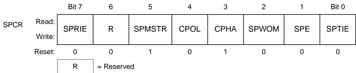
Figure 18-12. SPI Control Register (SPCR)
