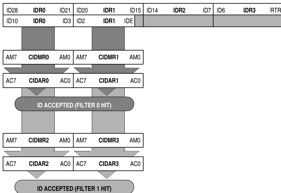
Figure 22-4. Dual 16-Bit Maskable Acceptance Filters
