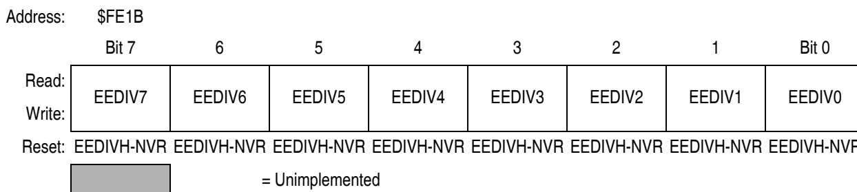
Figure 27-2. EEPROM-2 Divider Low Register (EEDIVL)
