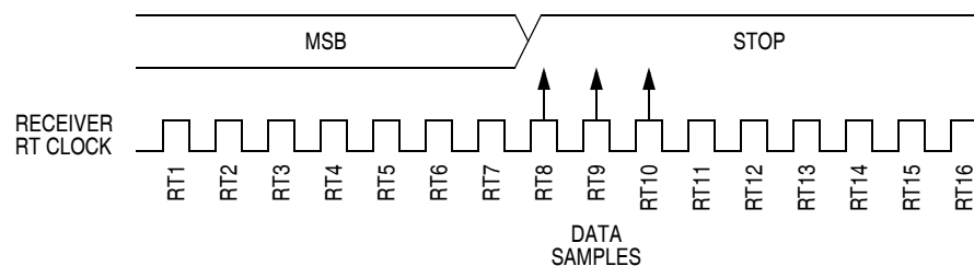
Figure 17-9. Slow Data
