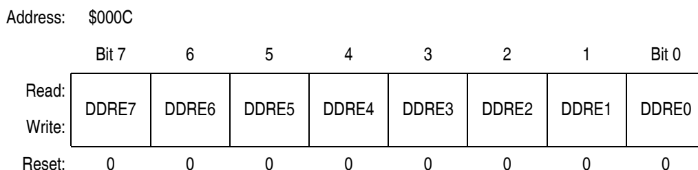
Figure 21-14. Data Direction Register E (DDRE)
