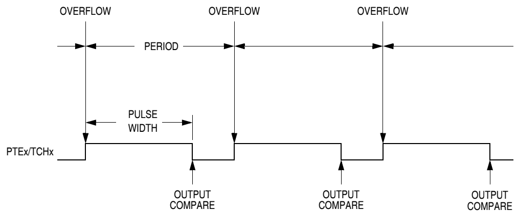
Figure 24-3. PWM Period and Pulse Width
