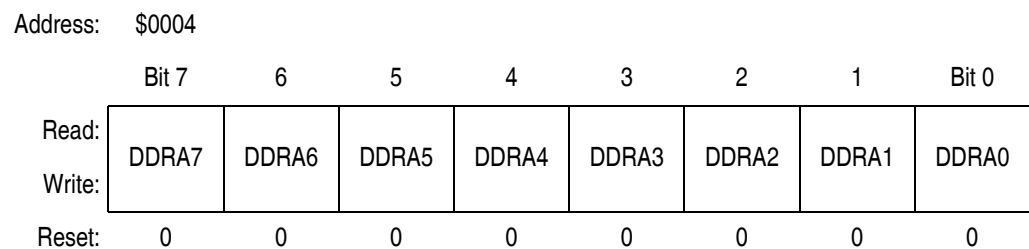
Figure 21-2. Data Direction Register A (DDRA)
