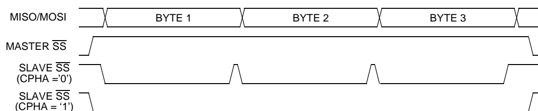
Figure 18-11. CPHA/ \overline{SS} Timing
