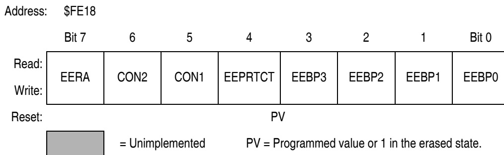
Figure 7-2. EEPROM-2 Nonvolatile Register (EENVR2)
