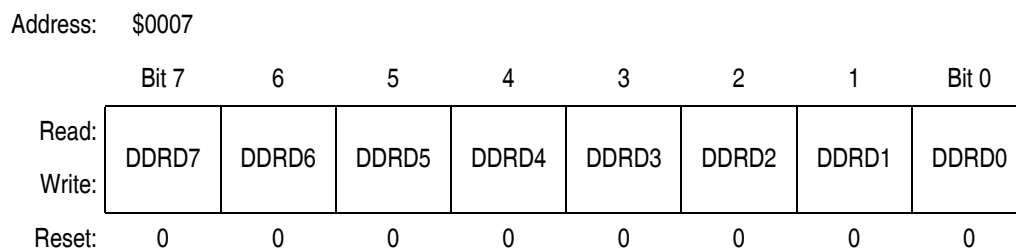
Figure 21-11. Data Direction Register D (DDRD)
