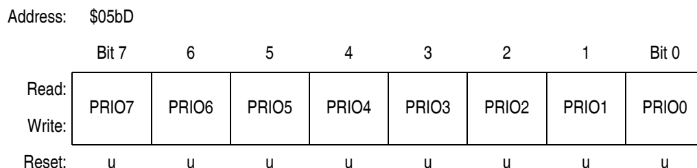
Figure 22-13. Transmit Buffer Priority Register (TBPR)
