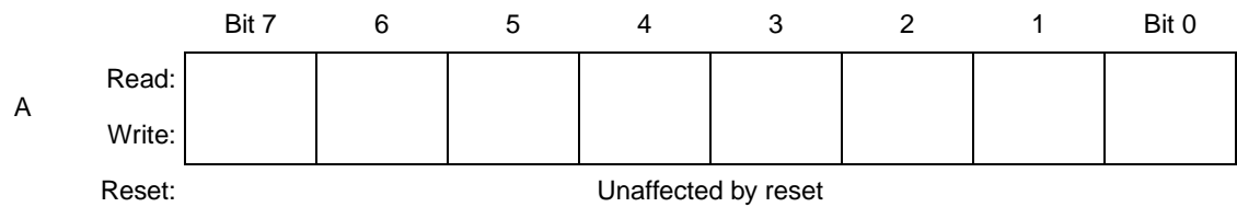
Figure 8-2. Accumulator (A)
