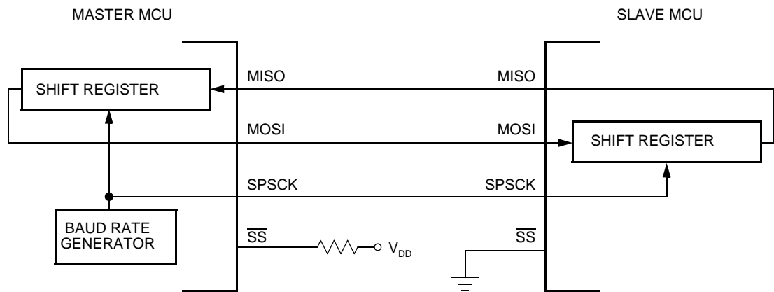
Figure 18-3. Full-duplex Master-Slave Connections
