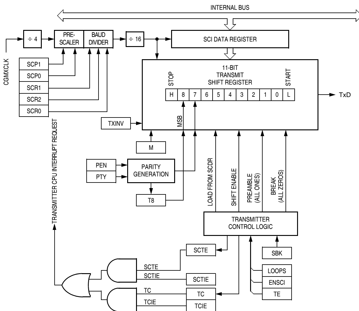
Figure 17-4. SCI Transmitter
