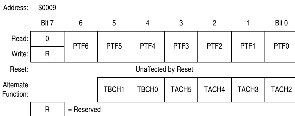
Figure 21-16. Port F Data Register (PTF)
