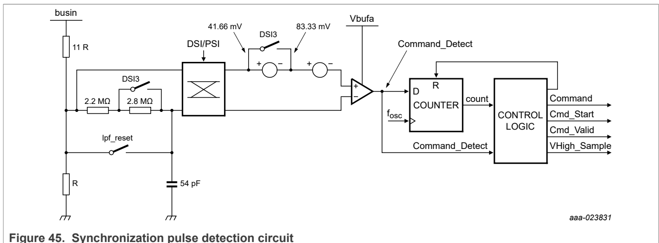
Figure 45. Synchronization pulse detection circuit
