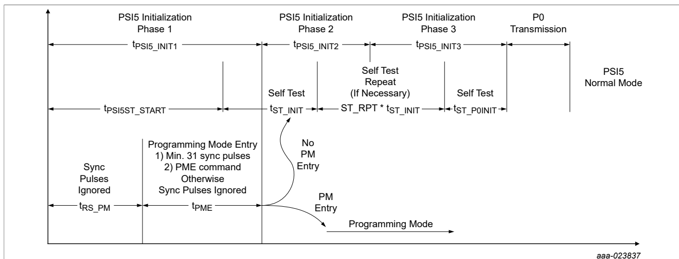
Figure 51. PSI5 initialization timing, synchronous mode
