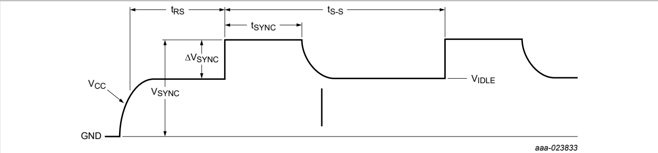
Figure 47. Sync pulse characteristics
