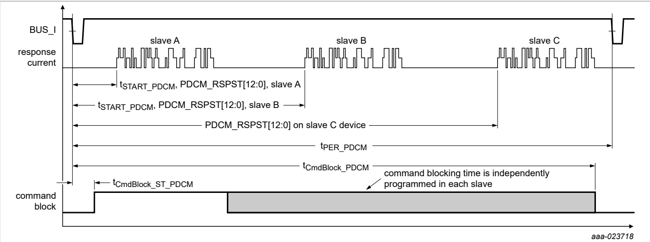
Figure 37. Periodic data mode response transmission
