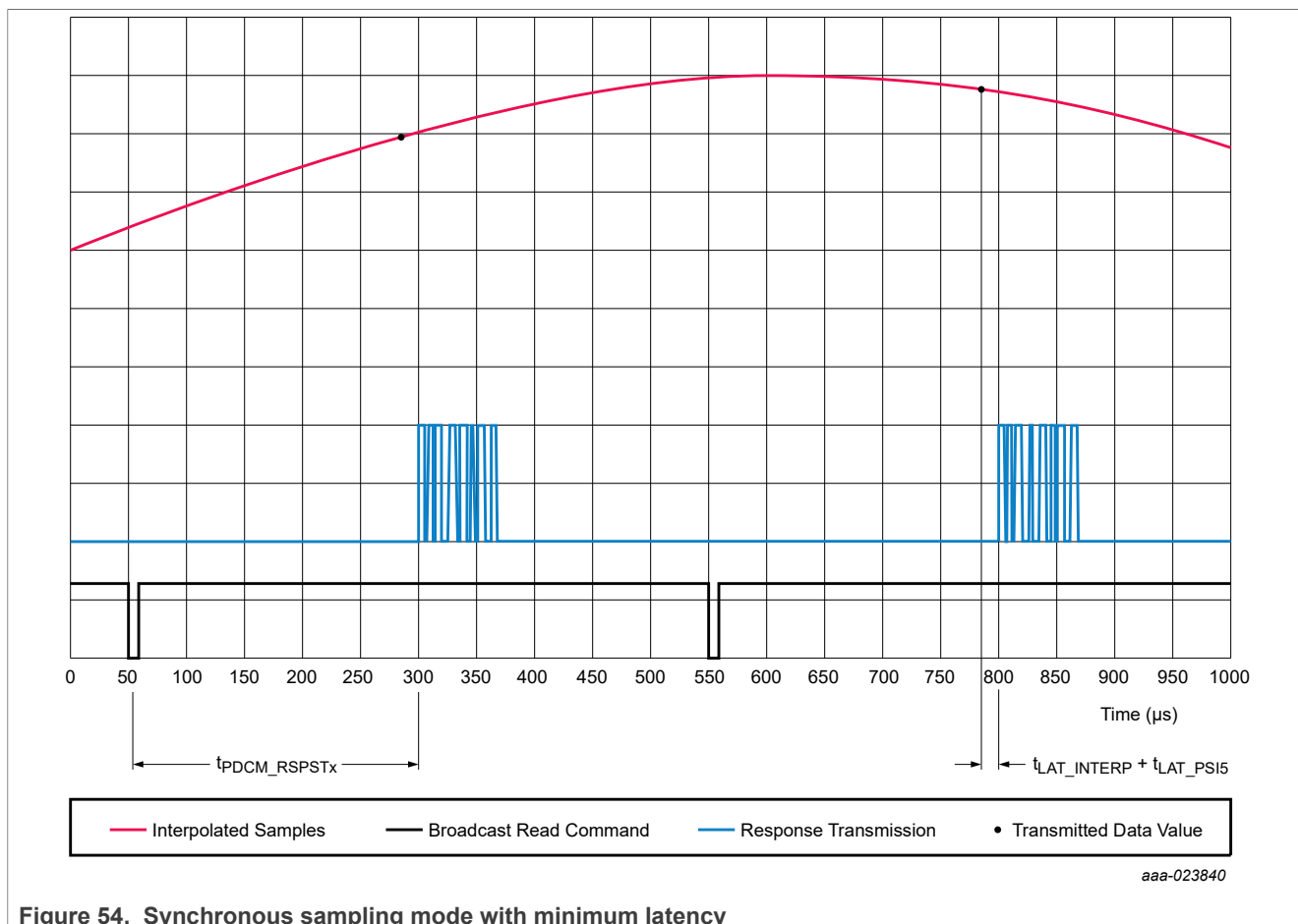
Figure 54. Synchronous sampling mode with minimum latency
