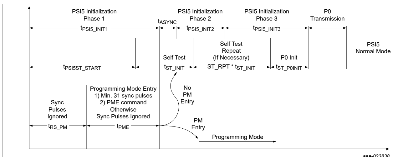
Figure 52. PSI5 initialization timing, asynchronous mode
