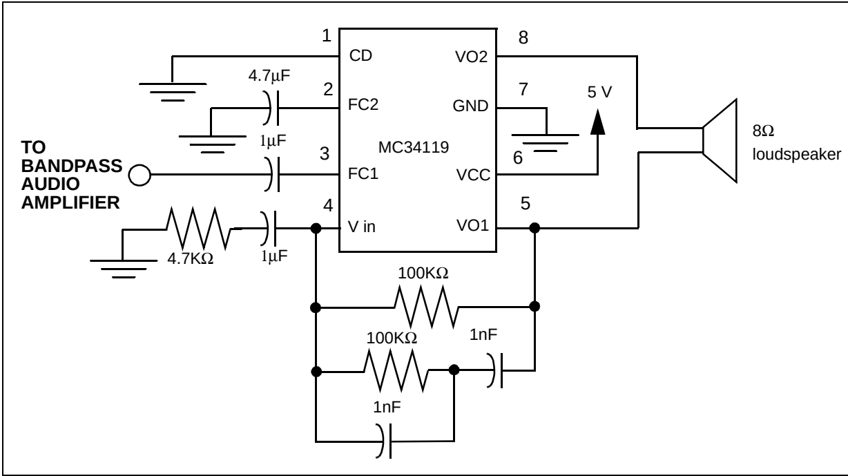
Figure 12. MC34119 Audio Amplifier in Banpass Configuration
