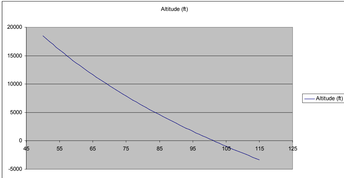
Figure 1. Pressure (kPa) vs. Altitude (ft)
