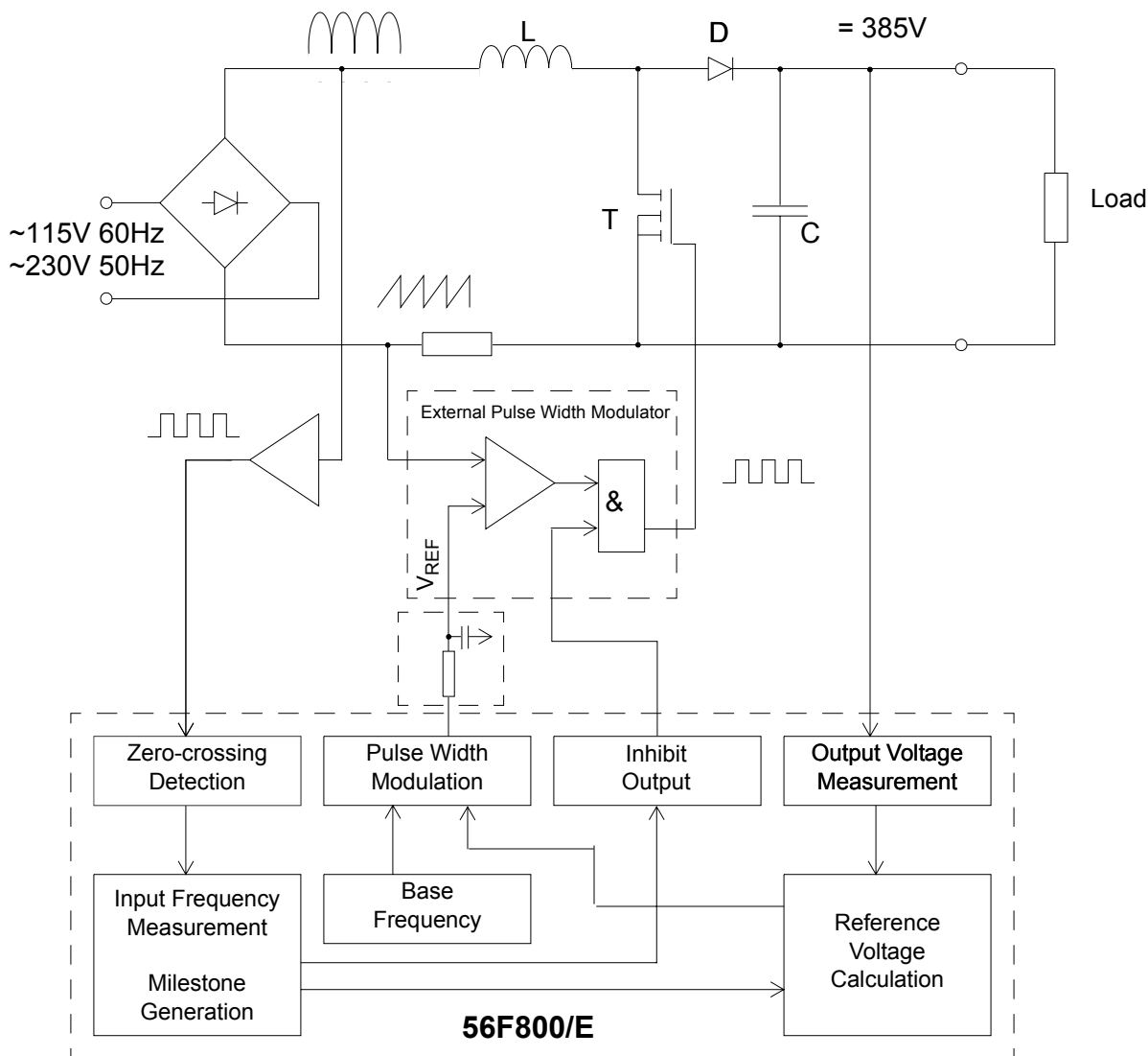
Figure 3-1. System Concept
