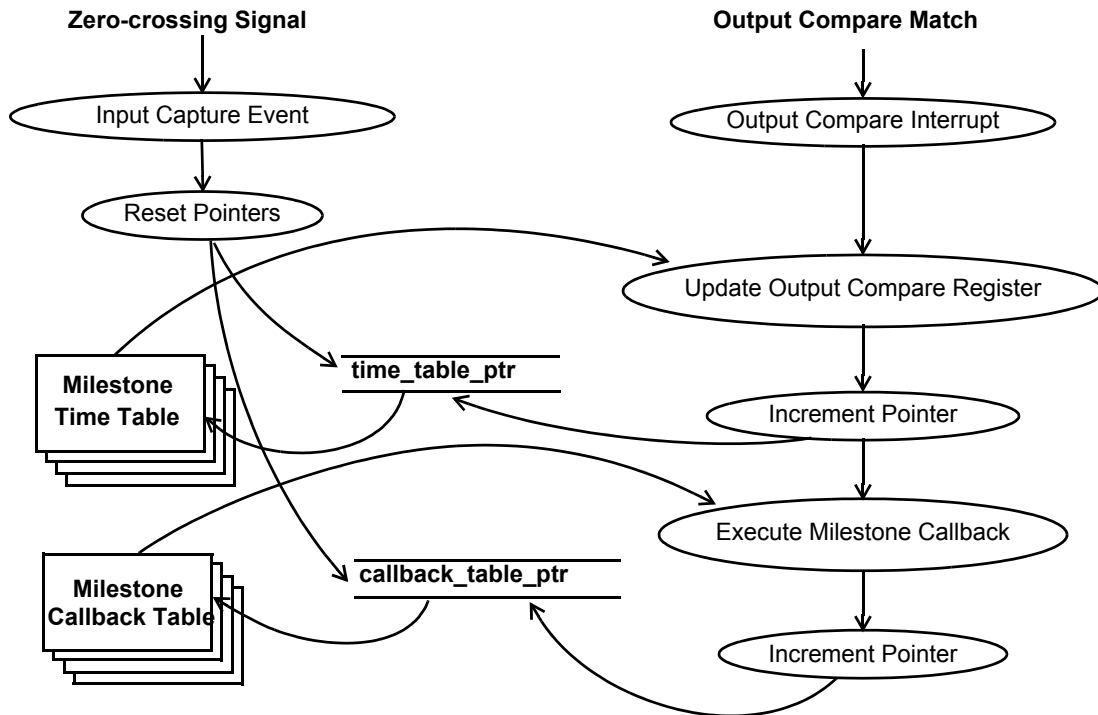
Figure 6-3. Milestone Generation
