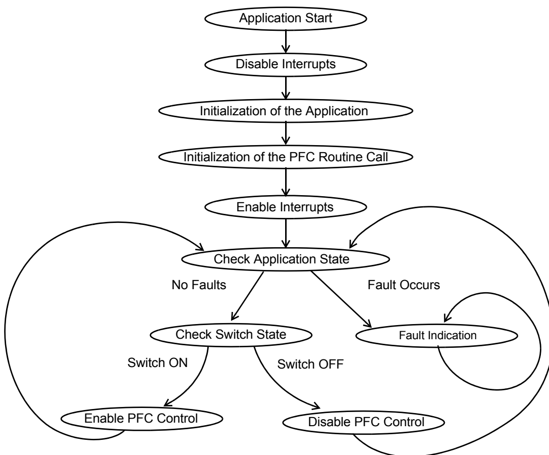
Figure 6-4. Application State Machine
