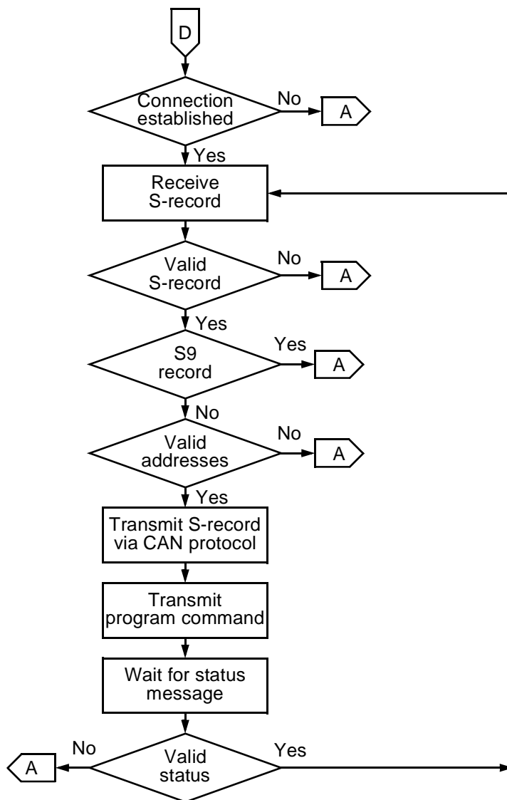
Figure 5. Smart cable process flow (Sheet 3 of 3)
