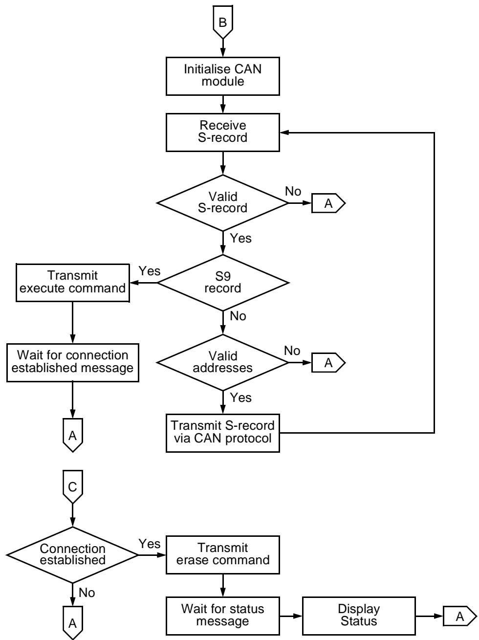
Figure 5. Smart cable process flow (Sheet 2 of 3)
