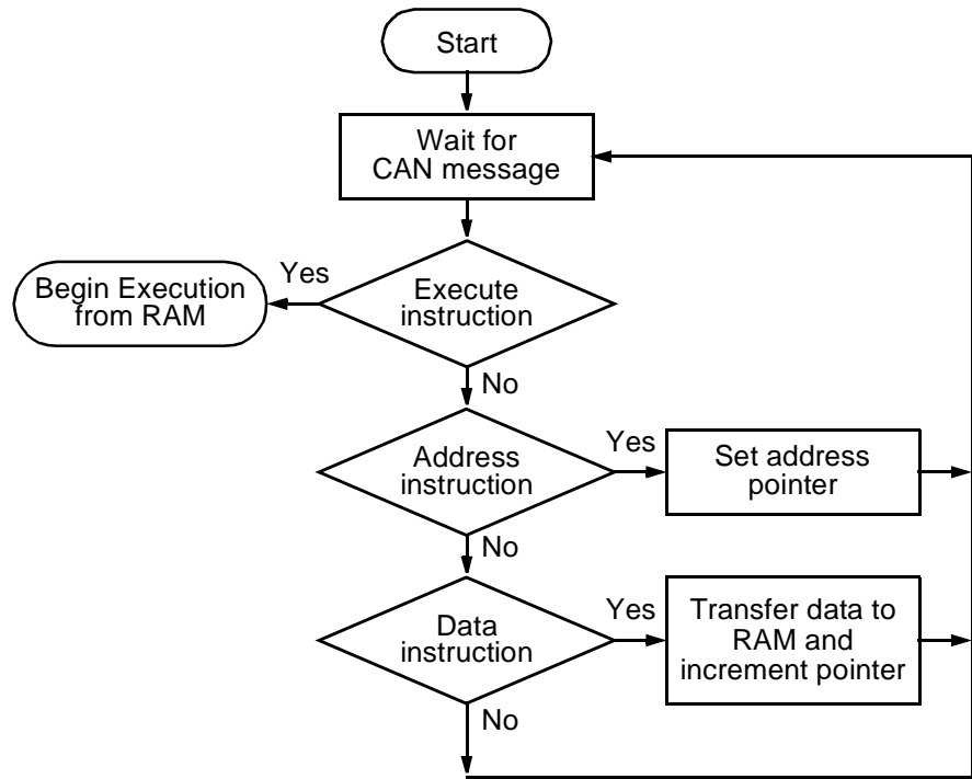
Figure 2. CAN load ram and execute process flow
