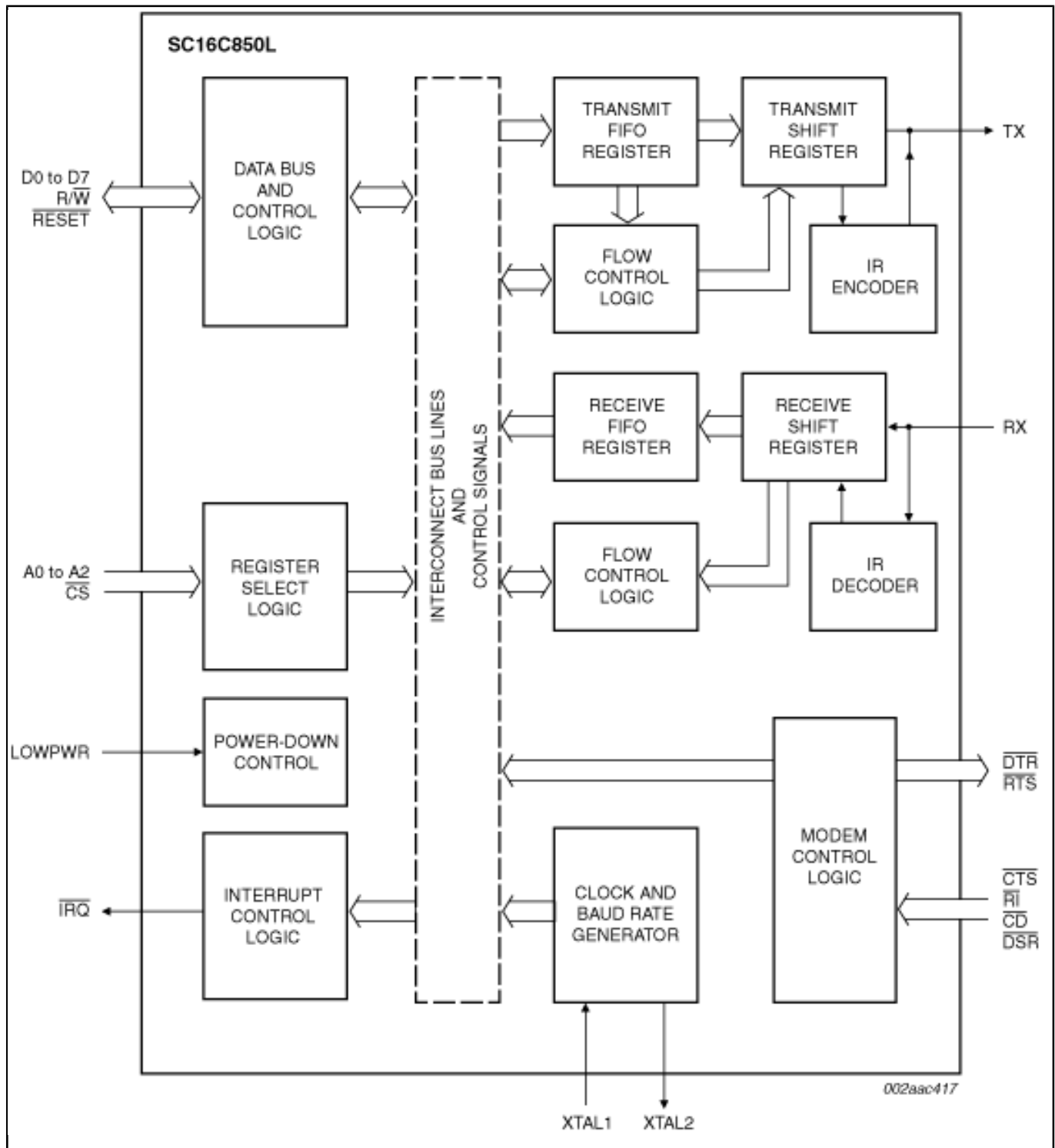
SC16C850LIB, SC16C850LIBS, SC16C850LIET Block Diagram
